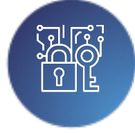
Cryptographic Security
